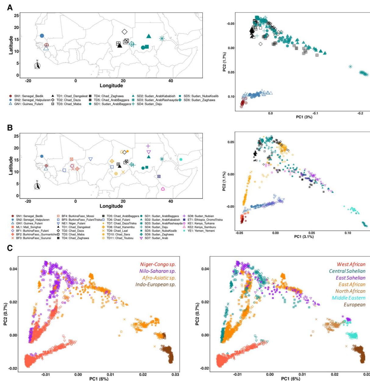
Fig. 1. Geographical locations and PCA for each assembled dataset. (A) Locations and PCA results for only Sahelian populations included in the present study. (B) Locations and PCA results of Sahelian populations across the Sahel/Savannah belt included in the present study and in previous studies (Triska et al. 2015; Haber et al. 2016; Vicente et al. 2019) (further details were included in supplementary fig. S2, Supplementary Material online). (C) PCA plots of worldwide populations included in the High-SNP density dataset (further details were included in supplementary fig. S4, Supplementary Material online). Populations were grouped according to their major linguistic affiliations (left plot) and geographical locations (right plot). Each PCA plot shows the first and second PC projections, and in parentheses the proportion of variance explained for each PC projection. Legend and further details about all the populations included in each dataset are detailed in supplementary fig. S3 and table S2, Supplementary Material online.
